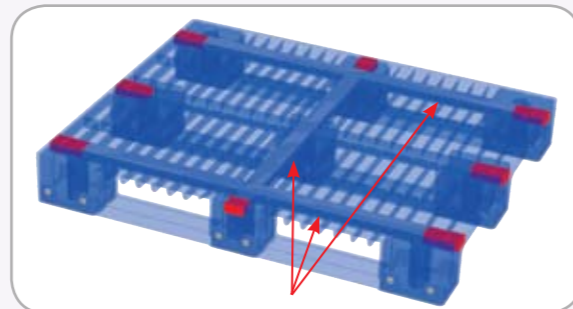
Width reinforcement
